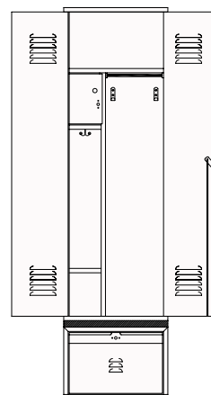
24" Wide/Drawer Base Welded or KD
